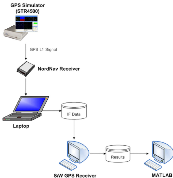
Fig. 4. Simulation Environment.
