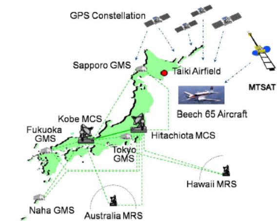
Fig. 1. MSAS system (Tsujii et al. 2008).
