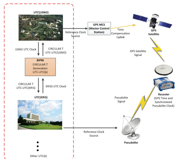
Fig. 1. UTC (KRIS) reference pseudolite time synchronization method.
