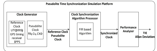
Fig. 3. Pseudolite time synchronization simulation platform.
