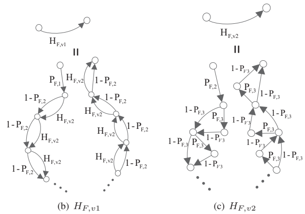
Fig. 4. Circular search diagram of proposed TSCLA technique-II.
