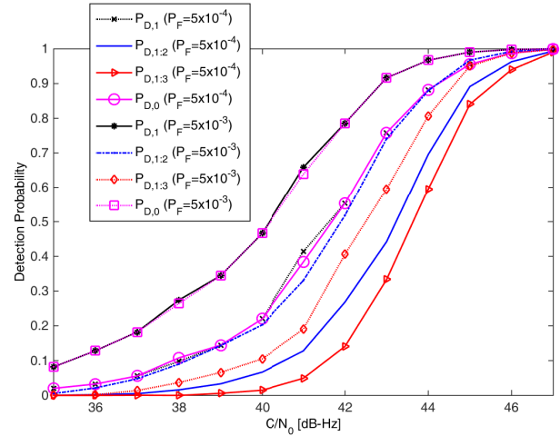
Fig. 5. Detection probability.
