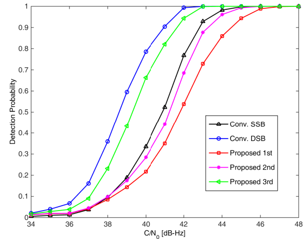
Fig. 7. Detection probability with respect to C/N_0 .
