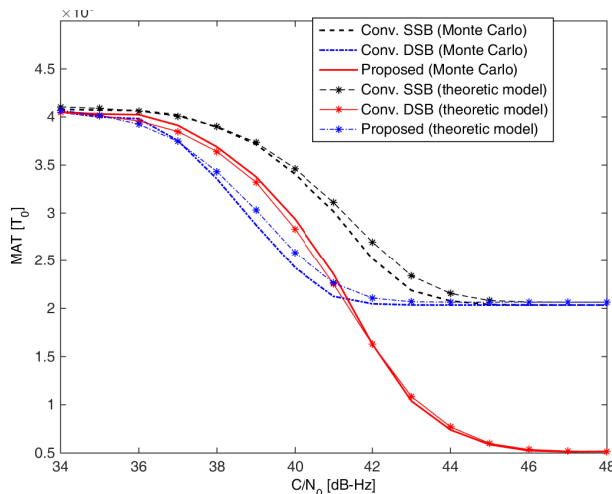
Fig. 8. Mean acquisition time with respect to C/N_0 .
