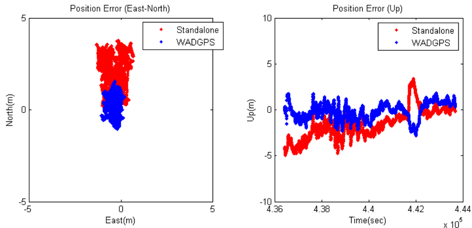
Fig. 9. Real-time positioning accuracy of static user (left: horizontal position error, right: vertical position error).
