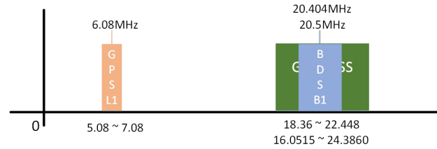
Fig. 7. A spectrum of 2nd frequency plan (LO frequency = 1581.5 MHz).
