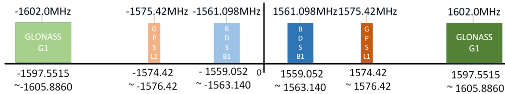
Fig. 1. The spectrum of GNSS signals on L1 band.
