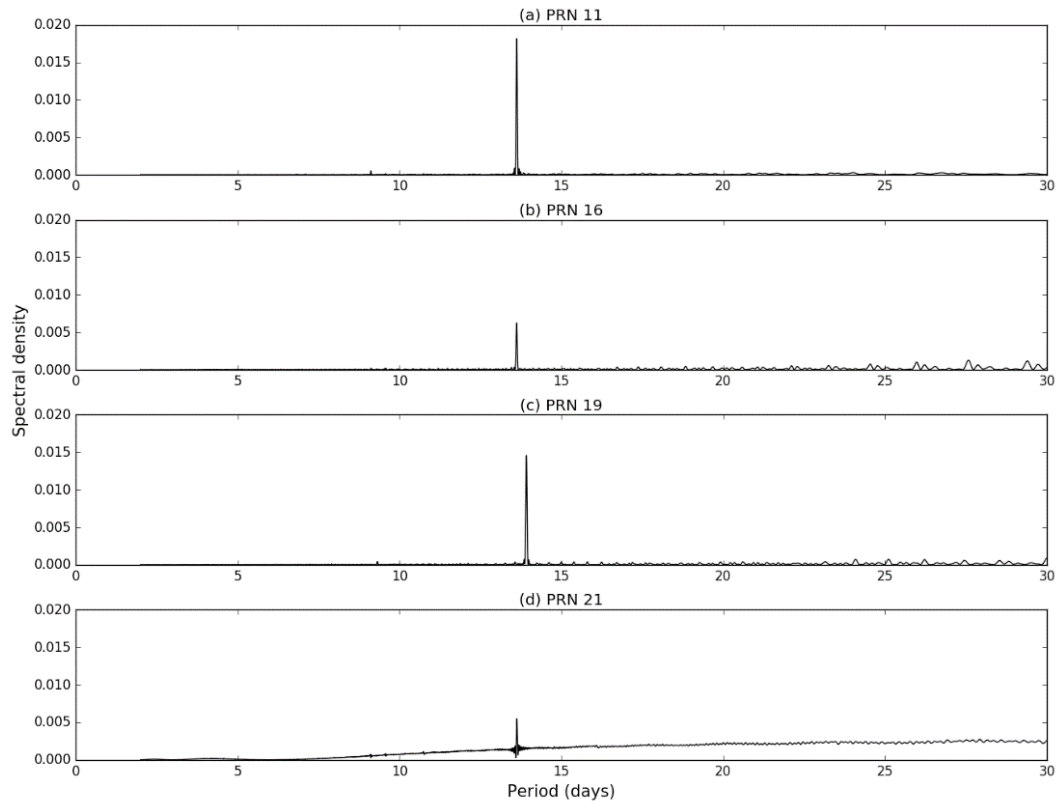
Fig. 3. Lomb-Scargle periodograms of sidereal shifts for (a) GPS PRN 11, (b) PRN 16, (c) PRN 19, and (d) PRN 21 from 2004 to 2014.
