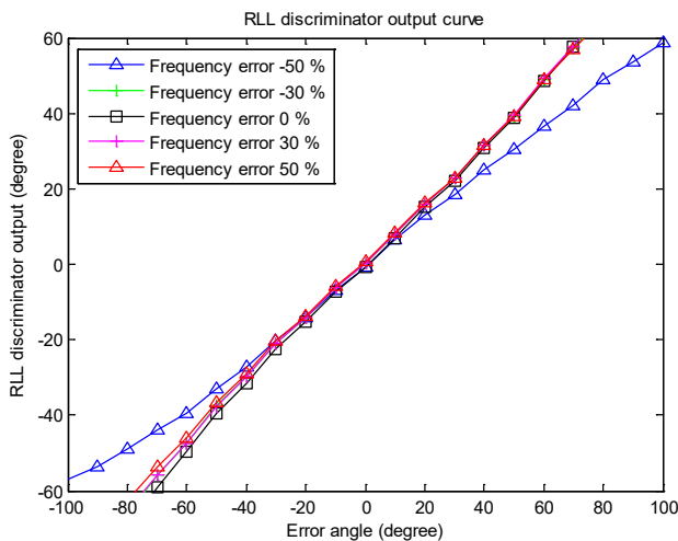
Fig. 8. RLL discriminator output curve w.r.t the rotation frequency error.
