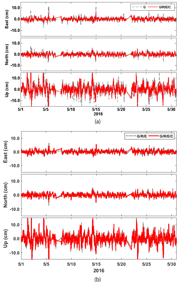
Fig. 4. Comparisons of GPS only, GPS+GLONASS+Galileo (G/R/E), and GPS+GLONASS+Galileo+BeiDou (G/R/E/C) kinematic PPP solutions at DAEJ station. (a) GPS only(G) and G/R/E/C, (b) G/R/E and G/R/E/C.
