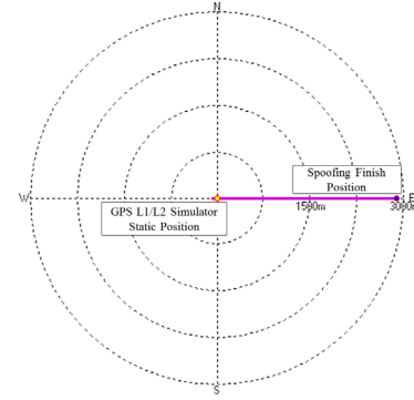
Fig. 9. Moving track of a commercial GPS receiver based on the spoofing injection scenario.
