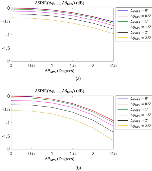
Fig. 2. The SINR degradation versus \Delta\theta_{\text{GPS}} for various values of \Delta\phi_{\text{GPS}} . (a) Single-polarized antenna array; (b) Dual-polarized antenna array.
