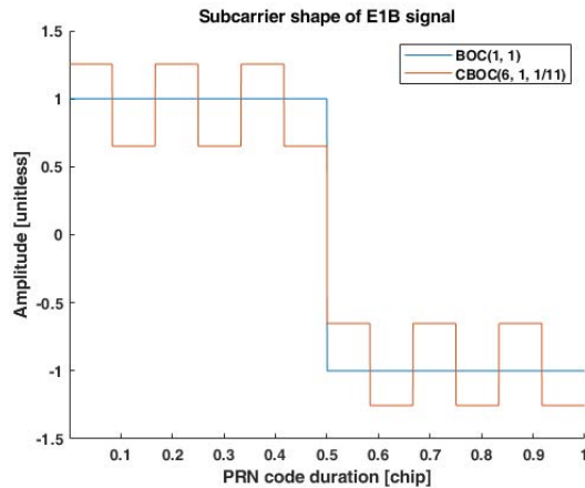
Fig. 3. The subcarrier shape of E1B signal.
