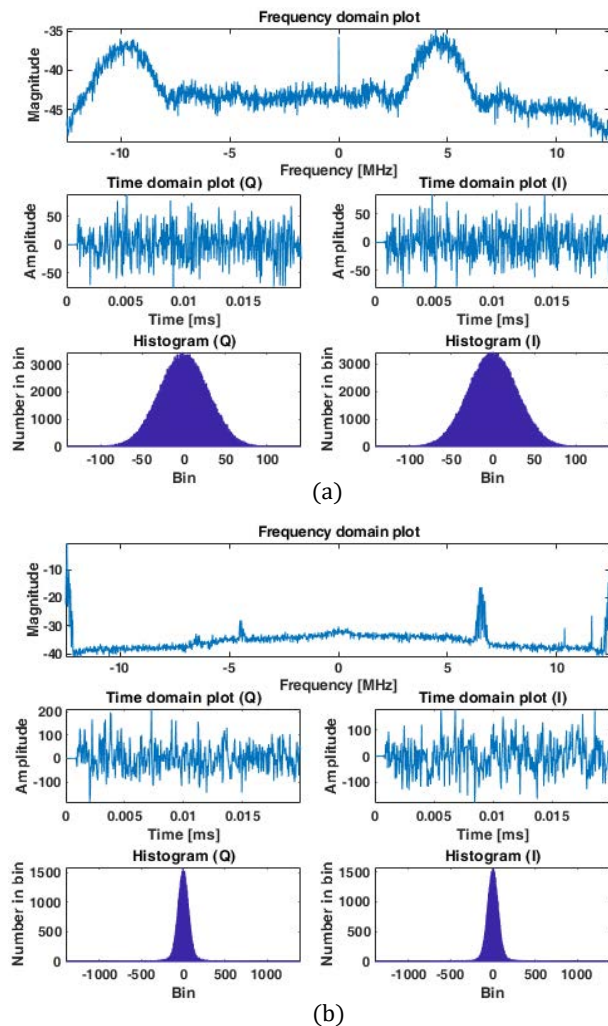
Fig. 6. Frequency & time domain plot and histogram of received signal: (a) L1 band, (b) L5 band.
