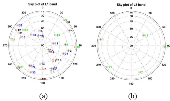
Fig. 10. Sky plots obtained from the introduced SDR: (a) L1 band, (b) L5 band. Each scenario is represented as different colors: Black is for GPS, Red is for QZSS, Blue is for BDS, Green is for Galileo.
