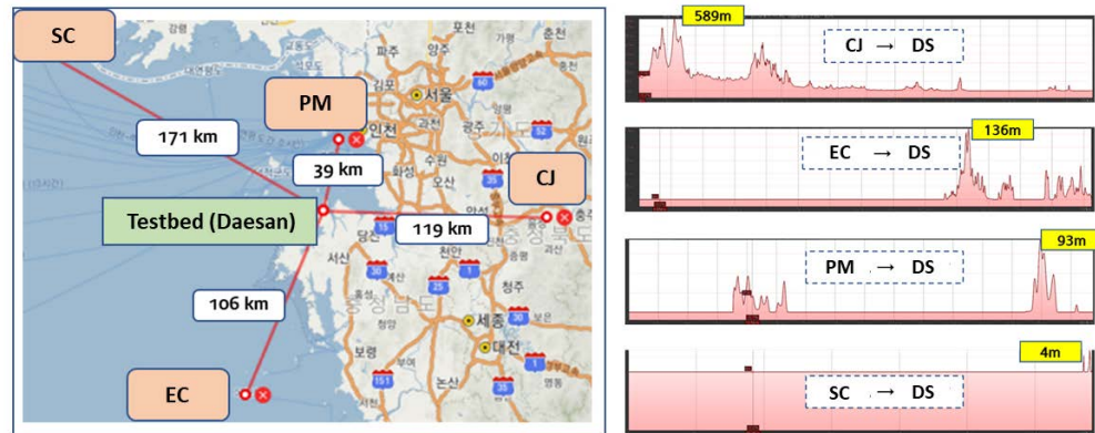
Fig. 3. Geometry of Korean MF R-Mode transmitting station and the Daesan testbed (left), The topographic characteristics of the propagation path of each MF R-Mode signal (right).
