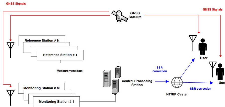
Fig. 1. Overall block diagram of POINT system.
