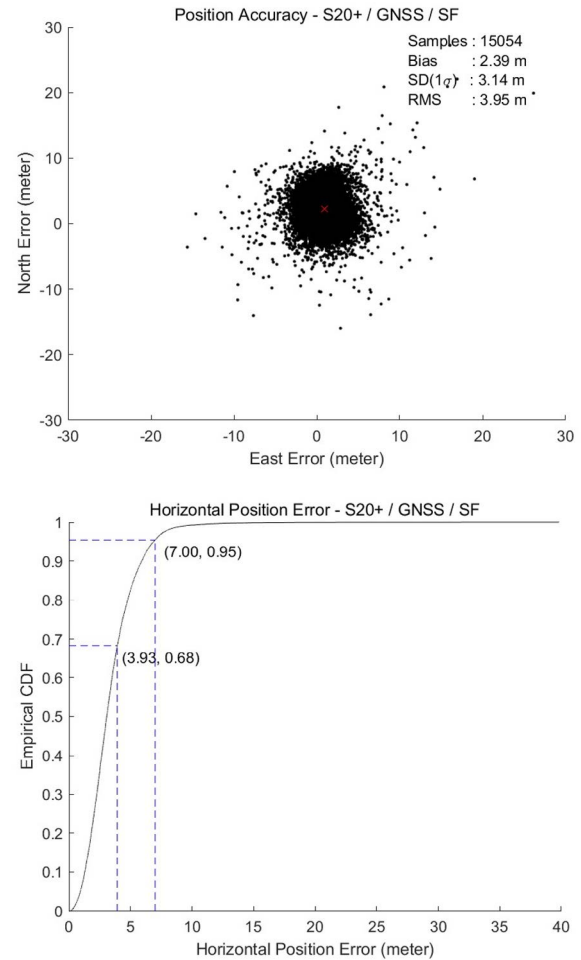
Fig. 6. Position accuracy – Horizontal position error.
