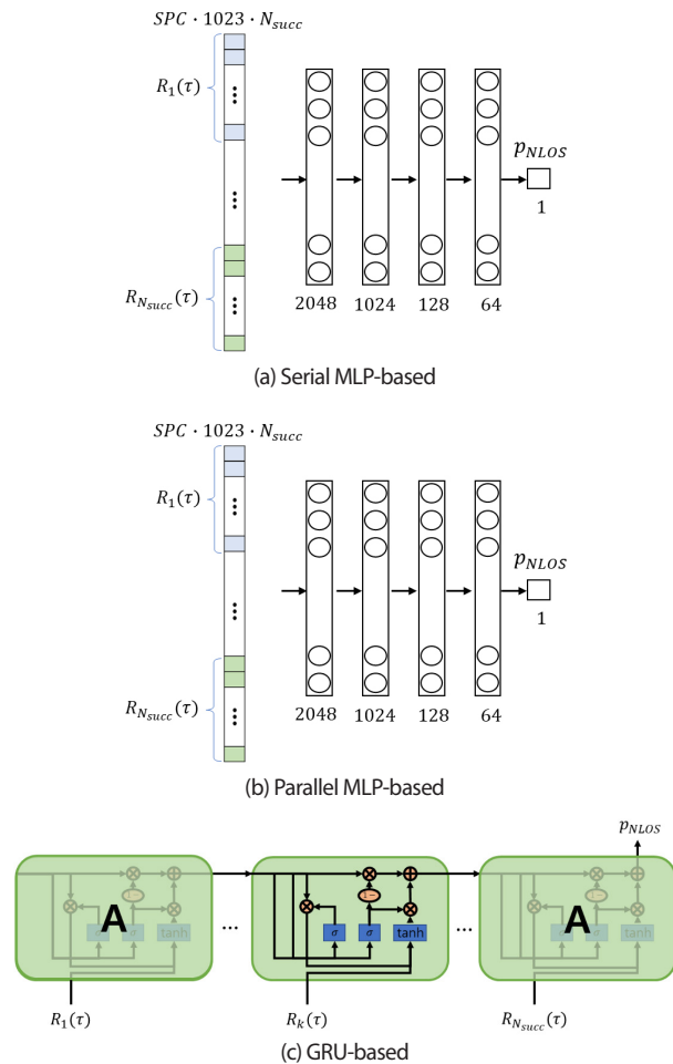
Fig. 9. MLP other NLOS signal classifier.
