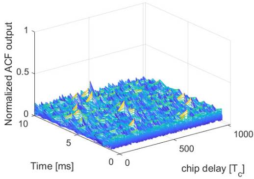
Fig. 7. auto-correlation function output examples with 3D plots and 2D heatmaps.
