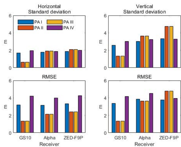
Fig. 10. Standard deviation and RMSE of four positioning algorithms for data set B.
